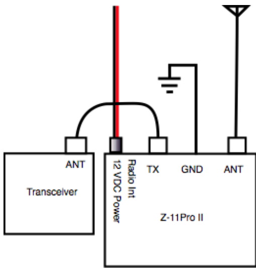
Typical Installation
